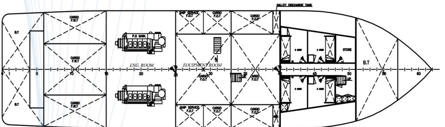
UNDER DECK
